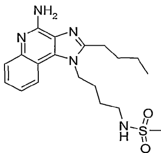
N -[4-(4-amino-2-butyl-1 H -imidazo[4,5- c ]quinolin-1-yl)butyl]methanesulfonamide;
